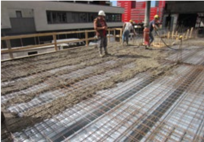
Concrete pouring on Cofraplus® 220 filling first the ribs
